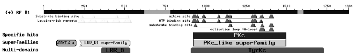
Fig. 3. Conserved domains of Ps SERK 1.
