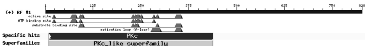
Fig. 4. Conserved domain of Pp SERK 2.
