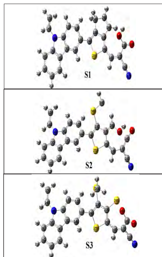
Structural sensitizers for dye-sensitized solar cells (dssc's): dft and td-dft investigation.
