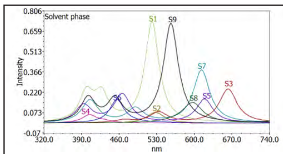
Figure 7: Calculated UV absorption spectra of the dyes in the acetonitrile solvent.
