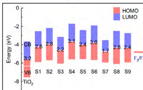
Figure 5: The energy gap ( E_g ) of the designed dyes S1 to S9 in a solvent.
