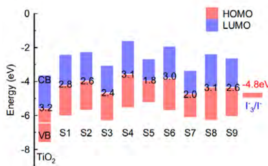
Figure 4: The energy gap ( E_g ) of the designed dyes S1 to S9 in the gas phase.
