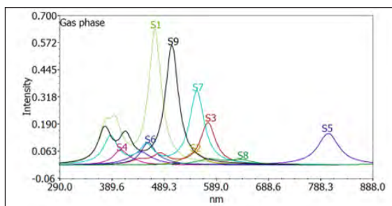
Figure 6: Calculated UV absorption spectra of the dyes in the gas phase.
