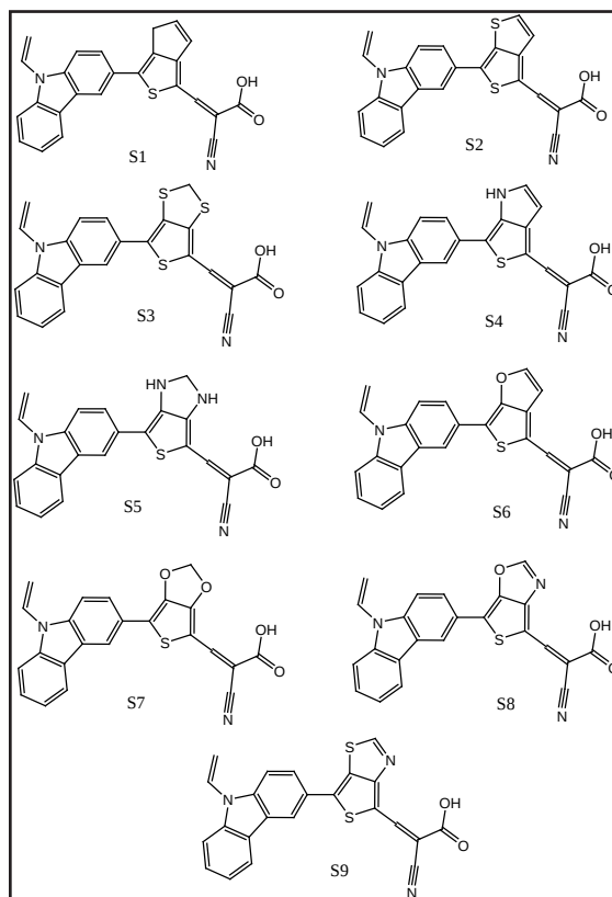
Figure 1: Molecular structure of the designed molecules (S1-S).
