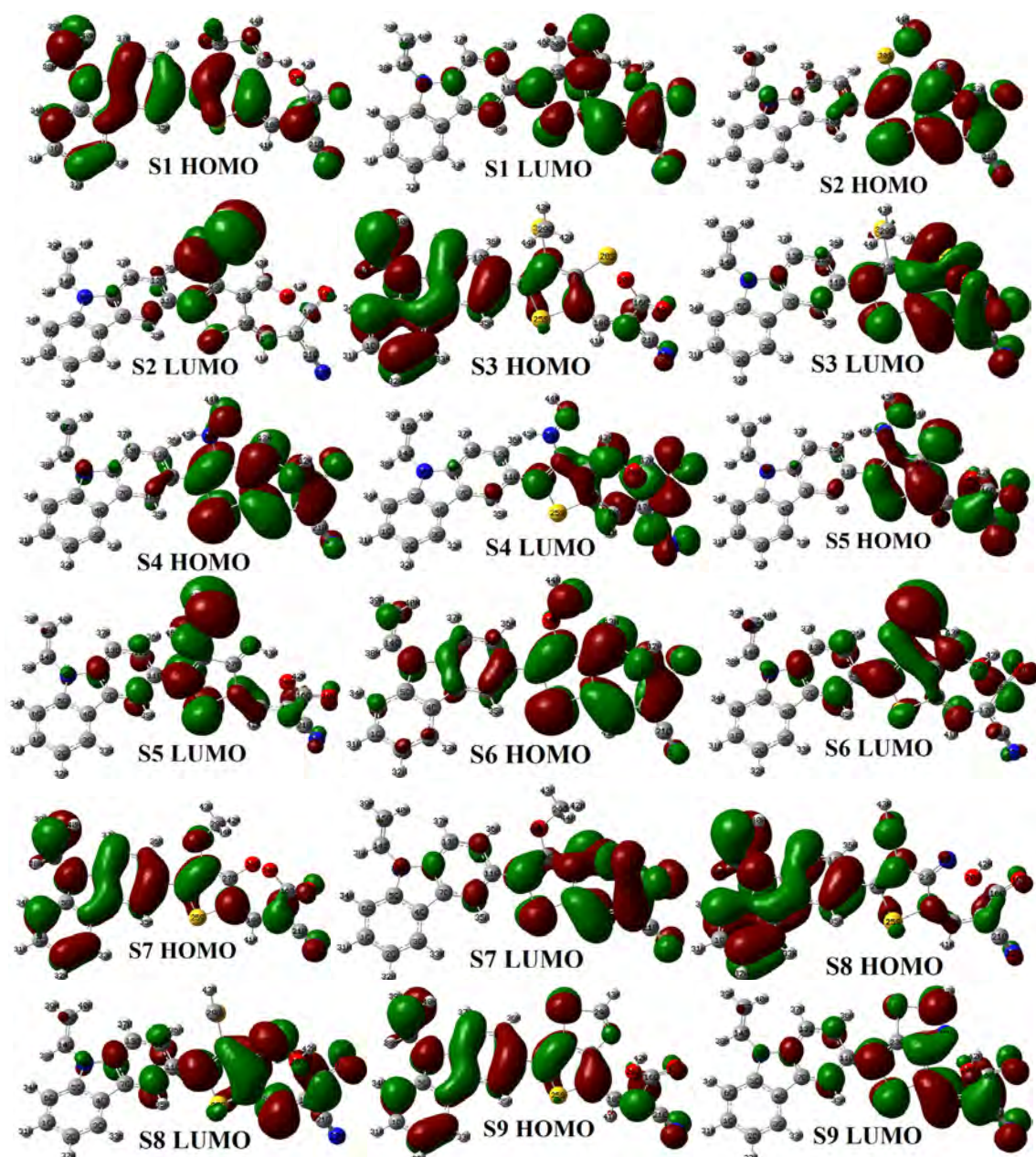
Figure 3: The HOMO and LUMO orbital diagrams for studied dyes S1 to S9 in the gas phase.
