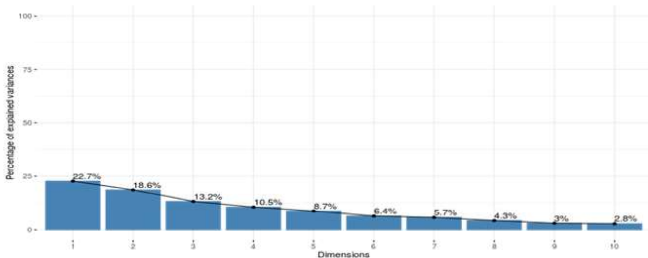
Fig 2. Scree plot
