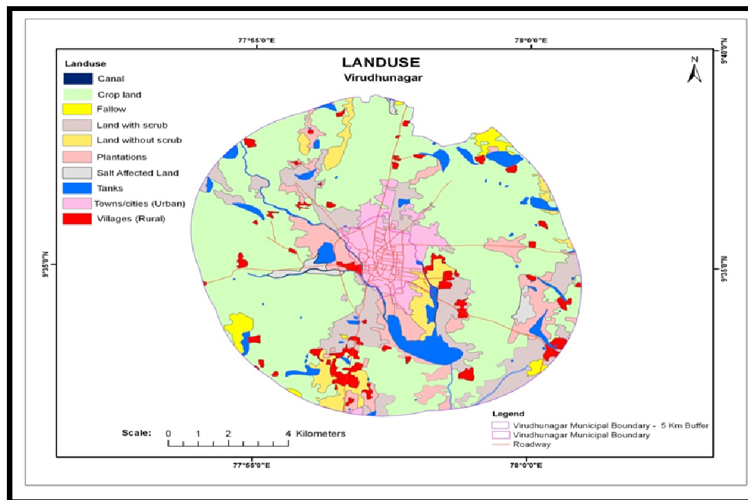
Figure 6: Landuse / land cover map of Virudhunagar Municipality with 5 km buffer.
