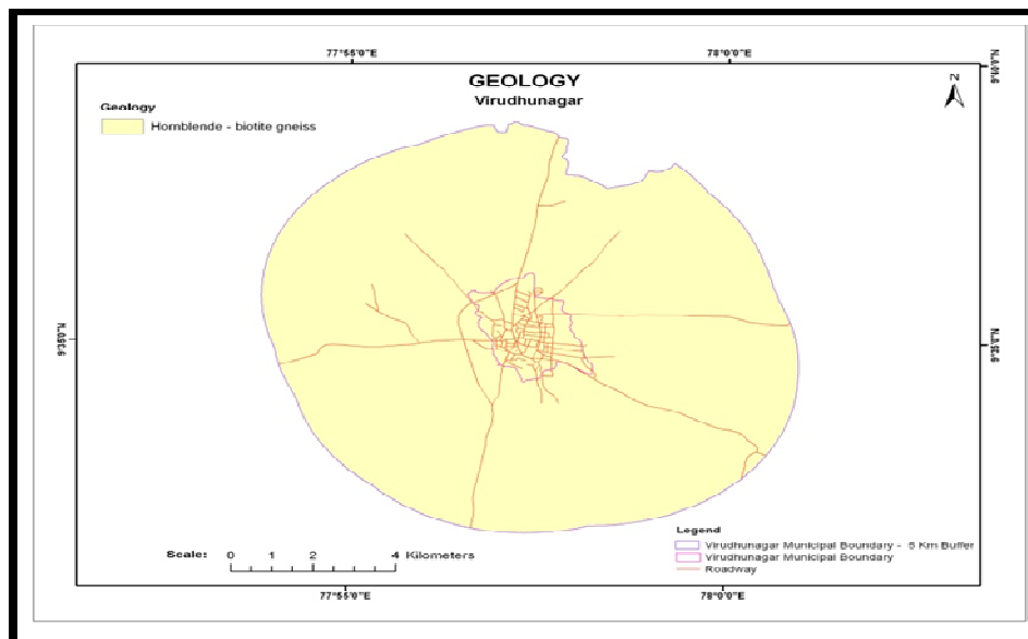
Figure 2: Geology map of Virudhunagar Municipality with 5 km buffer
