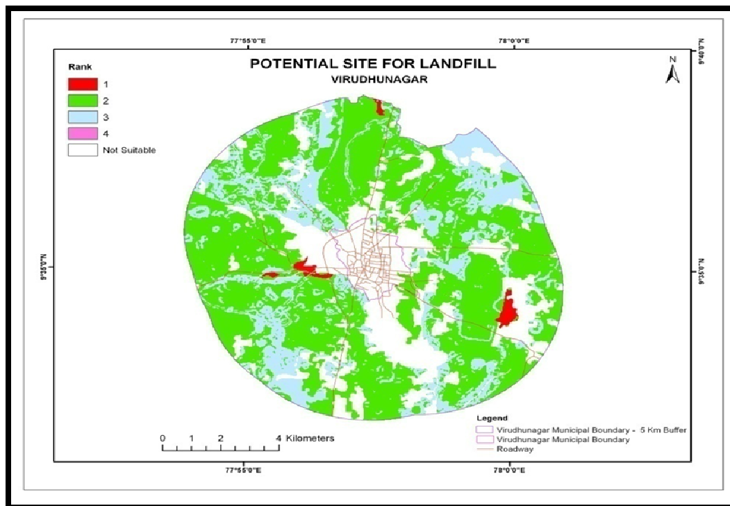
Figure 7: Suitable waste disposal sites in Virudhunager District
