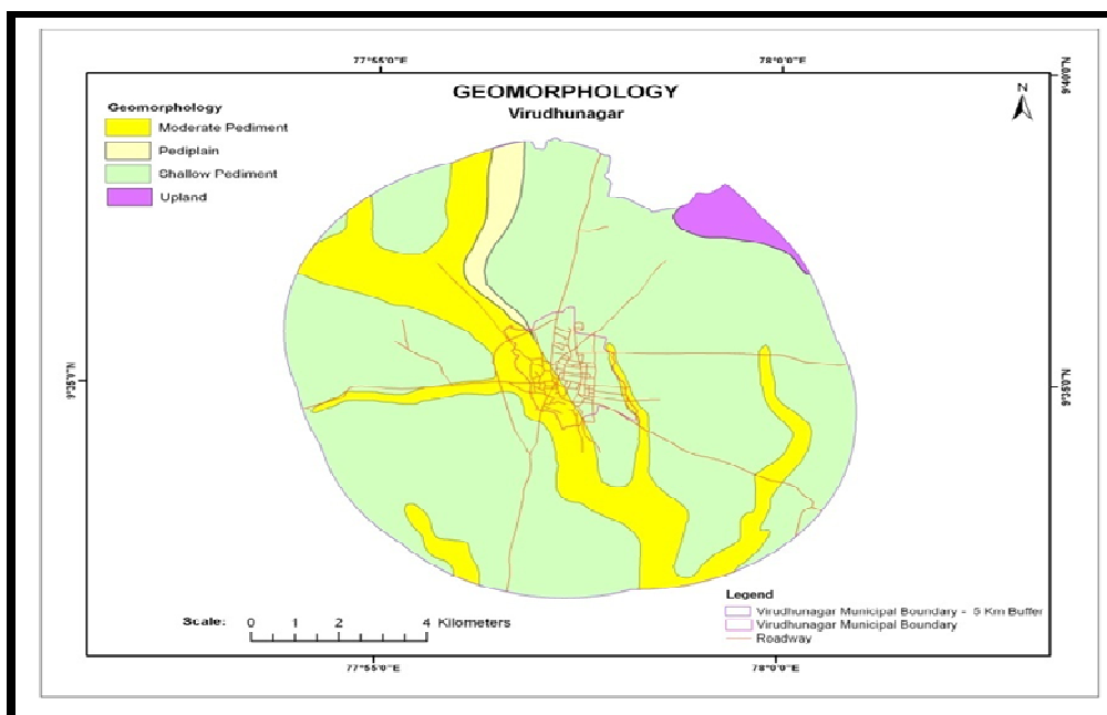
Figure 3: Geomorphology map of Virudhunagar Municipality with 5 km buffer
