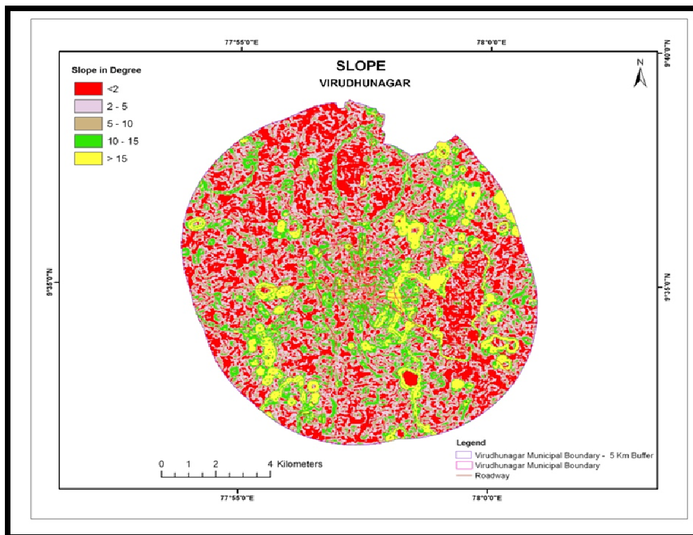
Figure 4: The Slope map of Virudhunagar Municipality with 5 km buffer
