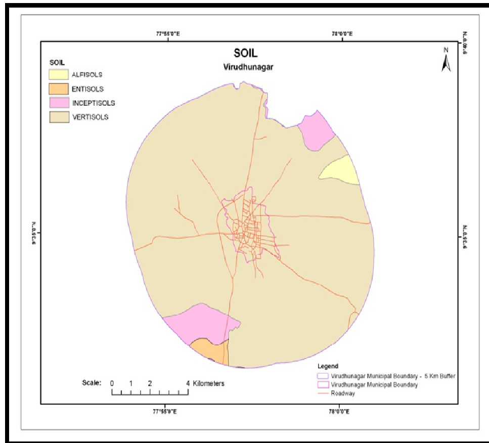
Figure 5: The soil map of Virudhunagar Municipality with 5 km buffer
