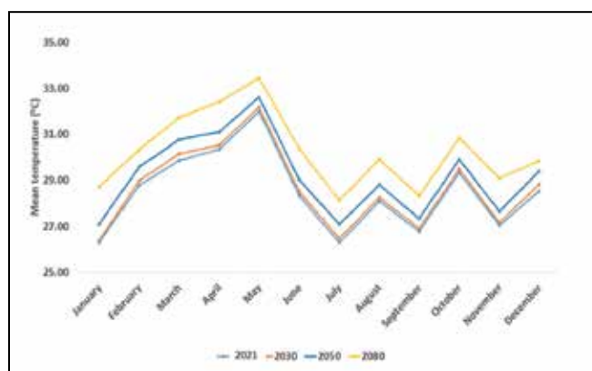
Figure 4: Monthly mean temperature ( ^{\circ}\text{C} ) during base line and future climates
