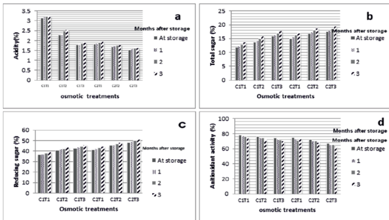
Fig 2. Changes in acidity (a), total sugar (b), reducing sugar(c) and antioxidant activity(d) of osmodehydrated G.gummi-gutta during storage
