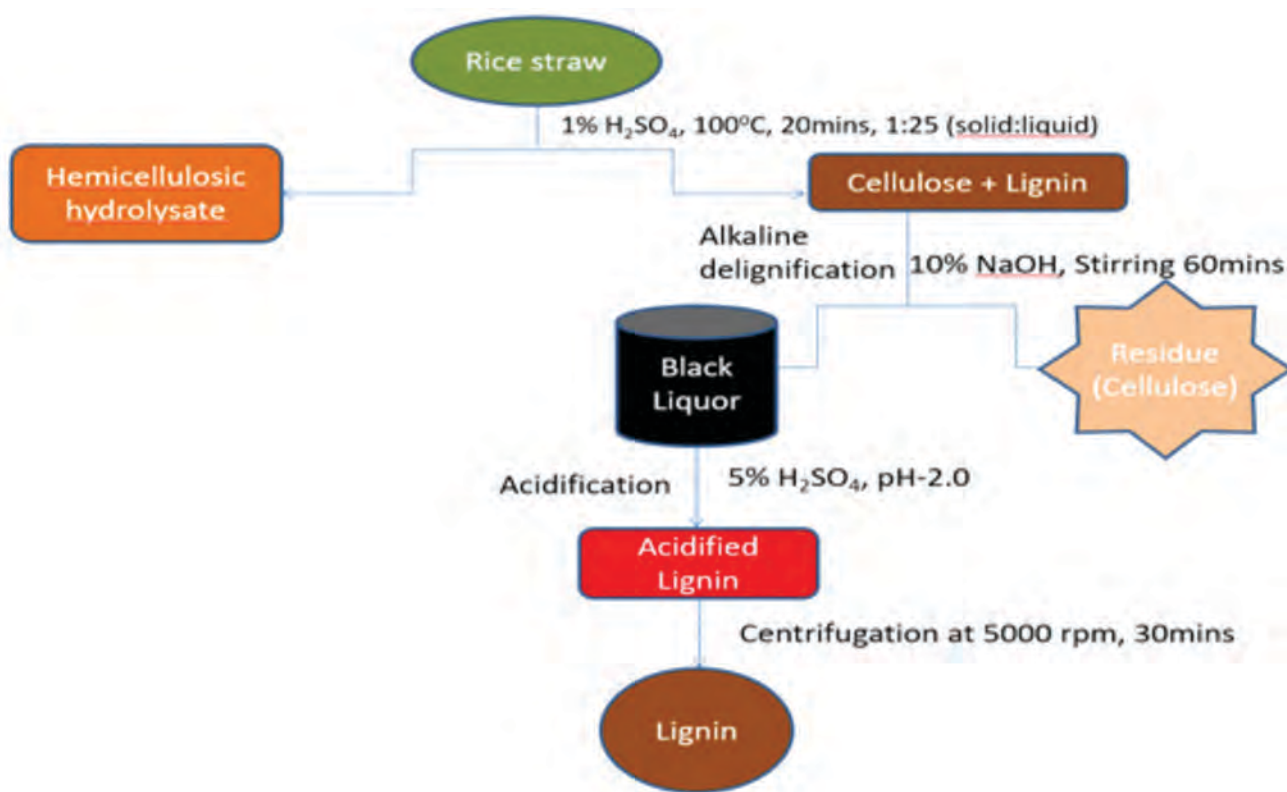
Fig. 1. Extraction of lignin from rice straw
