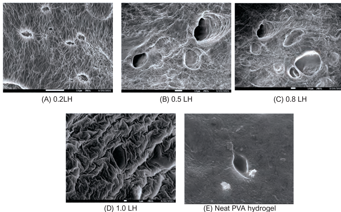
Fig. 2. SEM micrographs of different hydrogels LH: Lignin hydrogel
