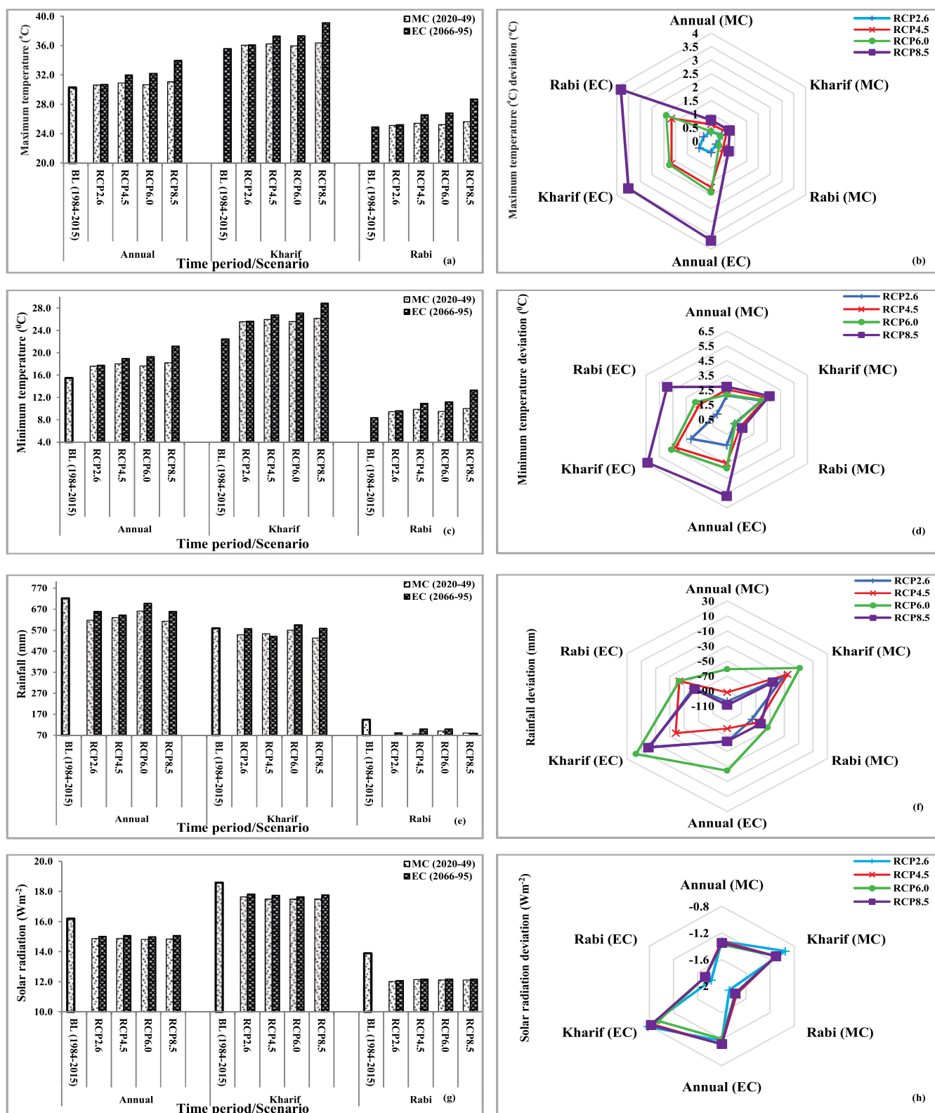
Fig. 4. Projected changes and deviation in (a and b) maximum temperature (°C), (c and d) minimum temperature (°C), (e and f) rainfall (mm) and (g and h) solar radiation (Wm -2 ) under different scenarios simulated by ensemble mean of five General Circulation Models at Amritsar (Agroclimatic zone III). # (BL: Baseline, EC: End-century, MC: Mid-century, RCP: Representative Concentration Pathway)
