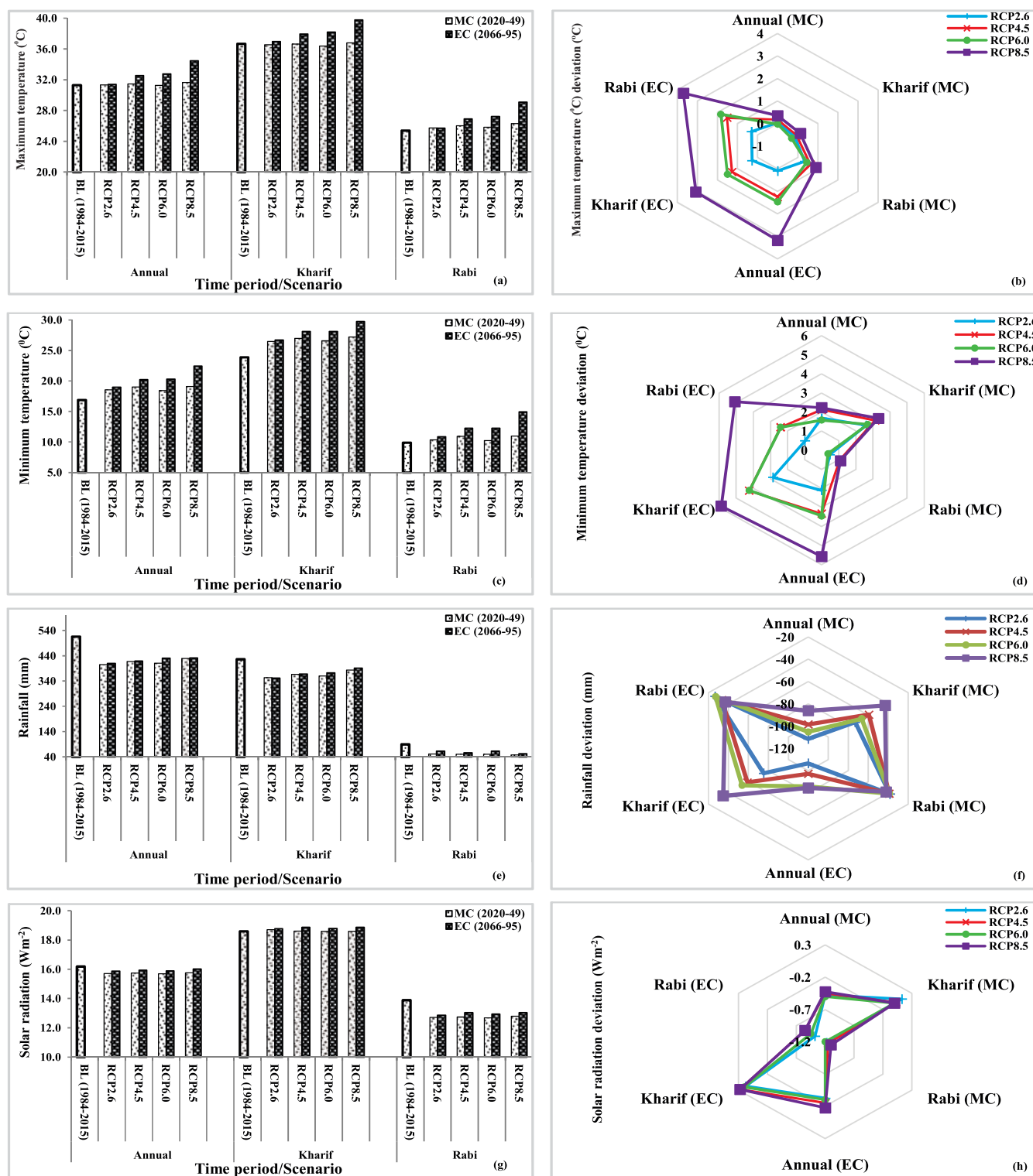
Fig. 6. Projected changes and deviation in (a and b) maximum temperature (°C), (c and d) minimum temperature (°C), (e and f) rainfall (mm) and (g and h) solar radiation (Wm -2 ) under different scenarios simulated by ensemble mean of five General Circulation Models at Bathinda (Agroclimatic zone IV). # (BL: Baseline, EC: End-century, MC: Mid-century, RCP: Representative Concentration Pathway)
