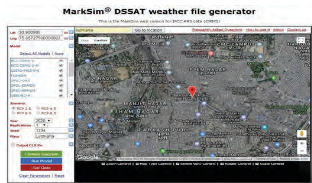
Fig. 1. MarkSim DSSAT weather generator Snapshot
