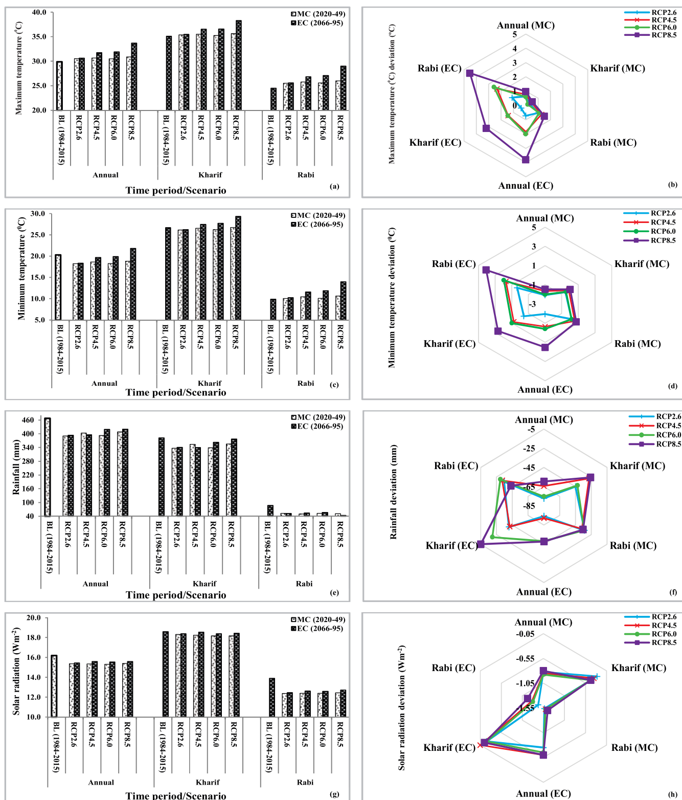
Fig. 8. Projected changes and deviation in (a and b) maximum temperature ( ^{\circ}\text{C} ), (c and d) minimum temperature ( ^{\circ}\text{C} ), (e and f) rainfall (mm) and (g and h) solar radiation ( \text{Wm}^{-2} ) under different scenarios simulated by ensemble mean of five General Circulation Models at Faridkot (Agroclimatic zone V). # (BL: Baseline, EC: End-century, MC: Mid-century, RCP: Representative Concentration Pathway)
