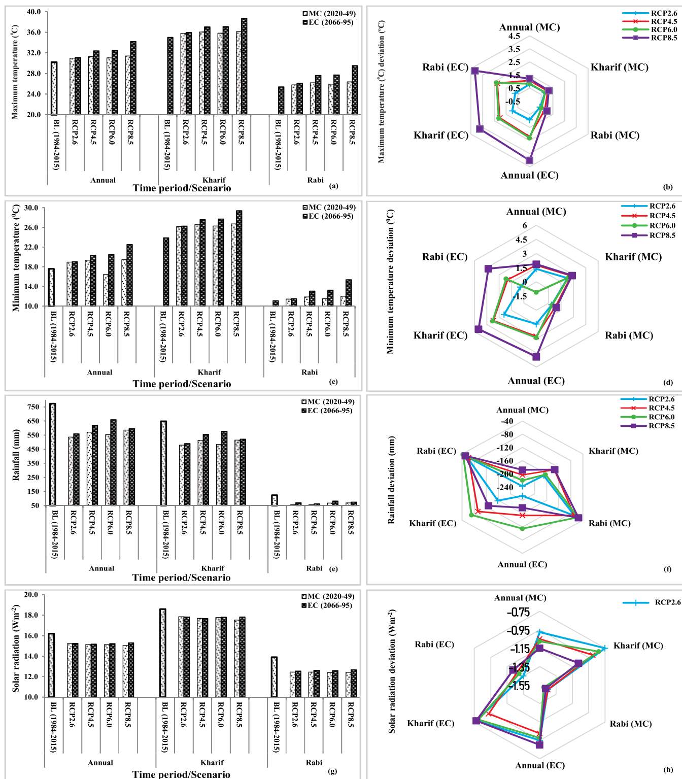
Fig. 5. Projected changes and deviation in (a and b) maximum temperature (°C), (c and d) minimum temperature (°C), (e and f) rainfall (mm) and (g and h) solar radiation (Wm -2 ) under different scenarios simulated by ensemble mean of five General Circulation Models at Patiala (Agroclimatic zone III). # (BL: Baseline, EC: End-century, MC: Mid-century, RCP: Representative Concentration Pathway)
