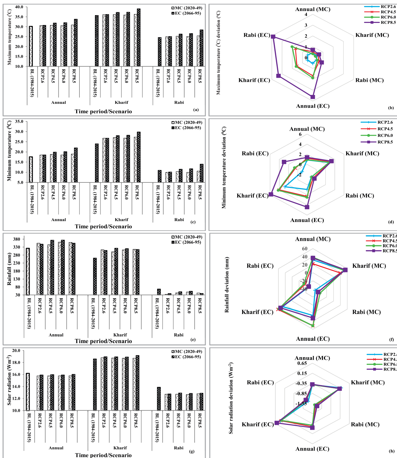
Fig. 7. Projected changes and deviation in (a and b) maximum temperature (°C), (c and d) minimum temperature (°C), (e and f) rainfall (mm) and (g and h) solar radiation (Wm -2 ) under different scenarios simulated by ensemble mean of five General Circulation Models at Abohar (Agroclimatic zone V). # (BL: Baseline, EC: End-century, MC: Mid-century, RCP: Representative Concentration Pathway)
