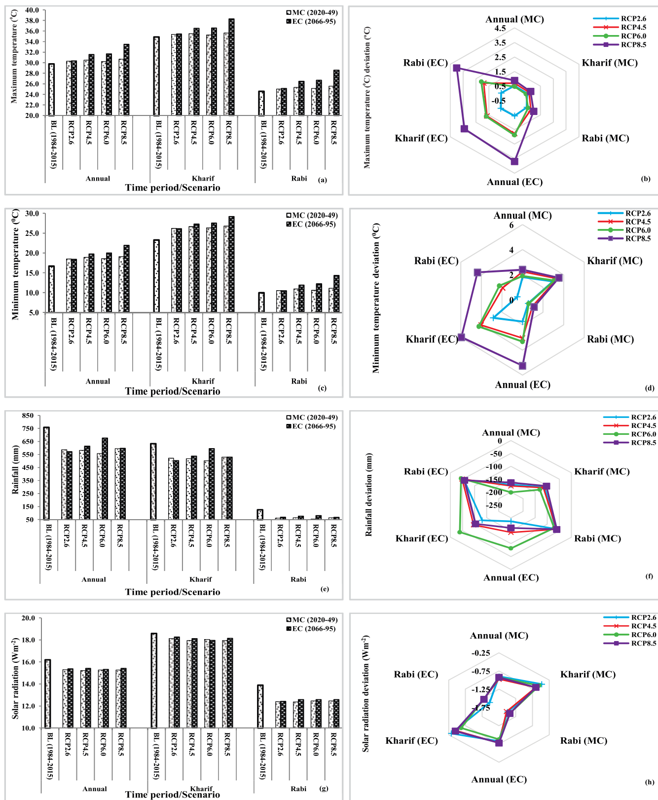
Fig. 3. Projected changes and deviation in (a and b) maximum temperature (°C), (c and d) minimum temperature (°C), (e and f) rainfall (mm) and (g and h) solar radiation (Wm -2 ) under different scenarios simulated by ensemble mean of five General Circulation Models at Ludhiana (Agroclimatic zone III). # (BL: Baseline, EC: End-century, MC: Mid-century, RCP: Representative Concentration Pathway)
