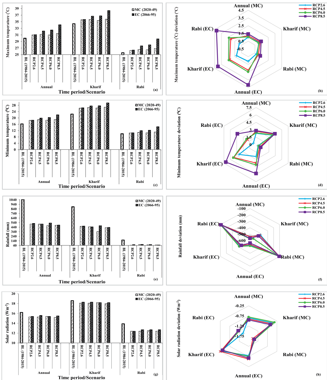
Fig. 2. Projected changes and deviation in (a and b) maximum temperature ( ^{\circ}\text{C} ), (c and d) minimum temperature ( ^{\circ}\text{C} ), (e and f) rainfall (mm) and (g and h) solar radiation ( \text{Wm}^{-2} ) under different scenarios simulated by ensemble mean of five General Circulation Models at Ballawal Saunkhri (Agroclimatic zone II). # (BL: Baseline, EC: End-century, MC: Mid-century, RCP: Representative Concentration Pathway)
