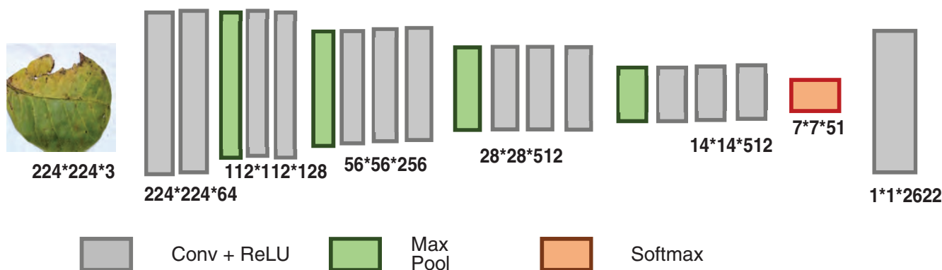
Fig. 2. VGG-16 architecture for feature extraction
