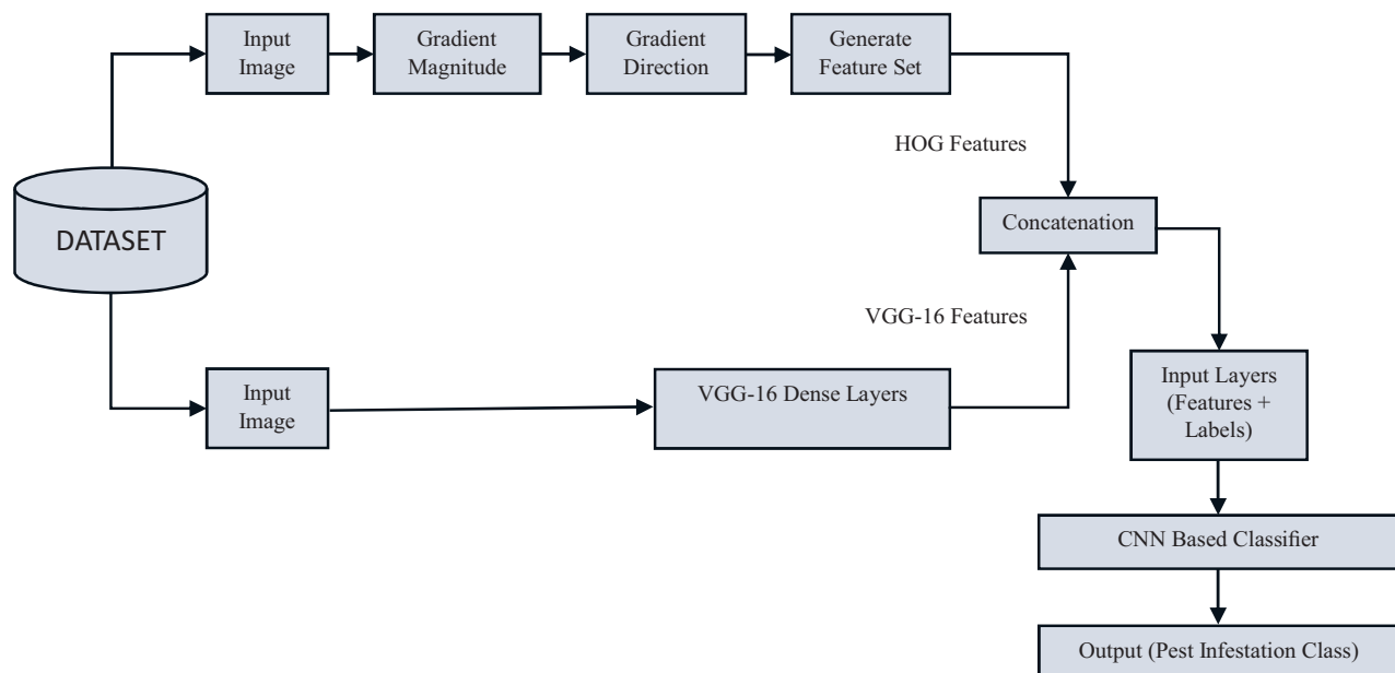
Fig. 3. Proposed model architecture
