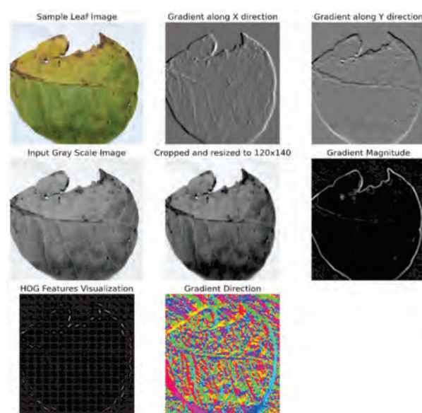
Fig. 1. Process to calculate gradient magnitude and direction
