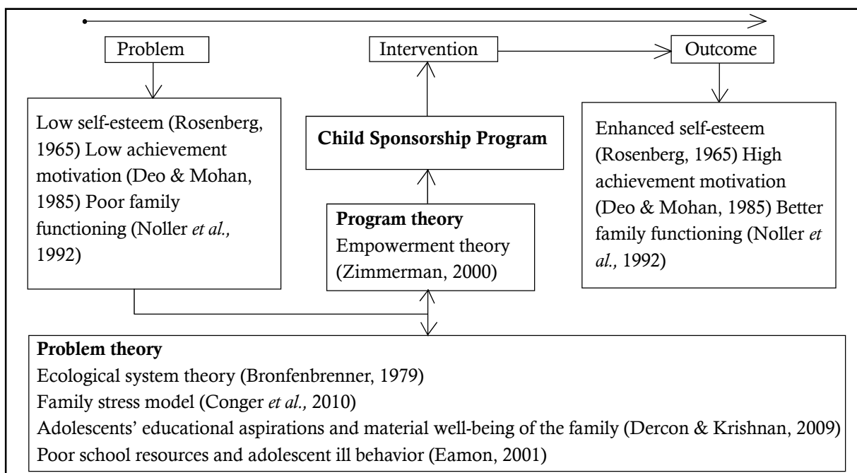
Figure 1. Theoretical Framework
